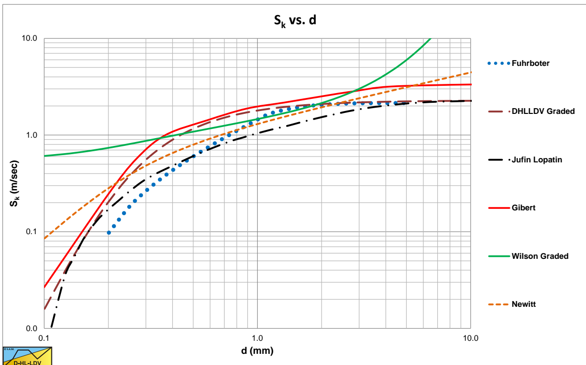
Figure 6.16-2 The S_k value of 6 models for D_p=0.2032 m, v_{ls}=4 m/s and C_{vt}=0.2 .
