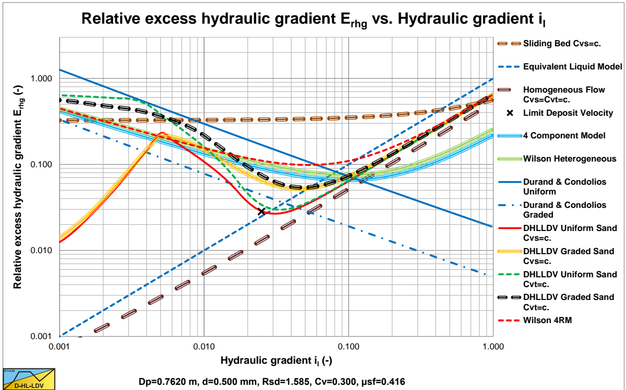
Figure 9.5-12: The resulting relative excess hydraulic gradient curves, also named the stratification ratio, D_p=0.762 m.
