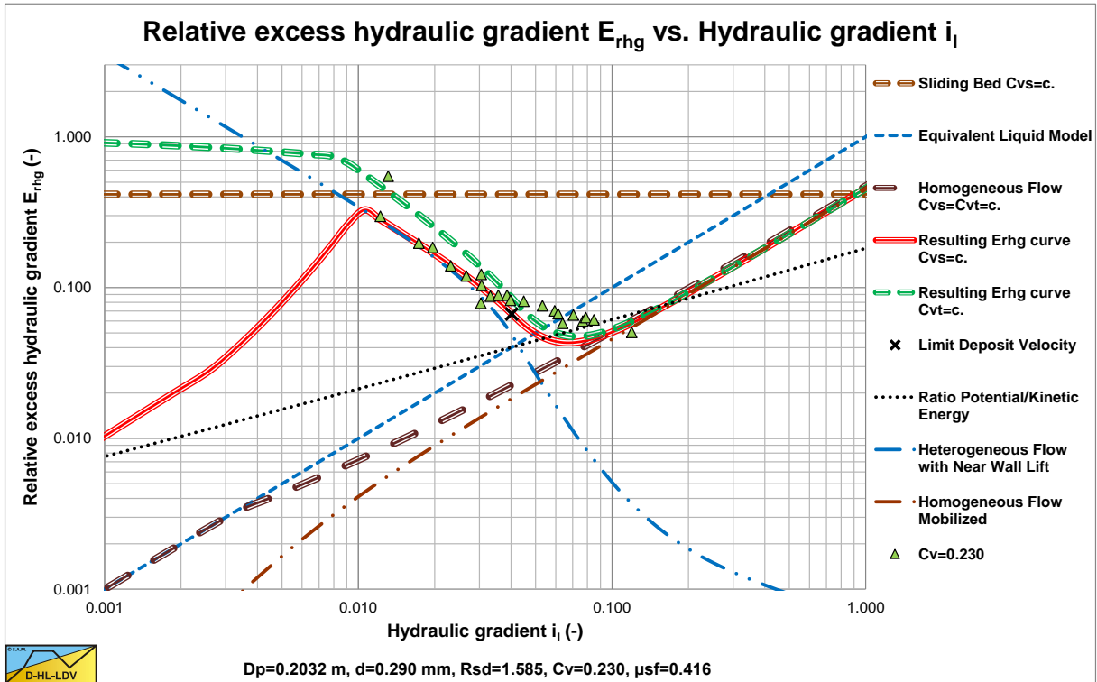
Figure 7.11-2: Experiments of Clift et al. (1982) in a 0.2082 m diameter pipe and a 0.29 mm particle.
