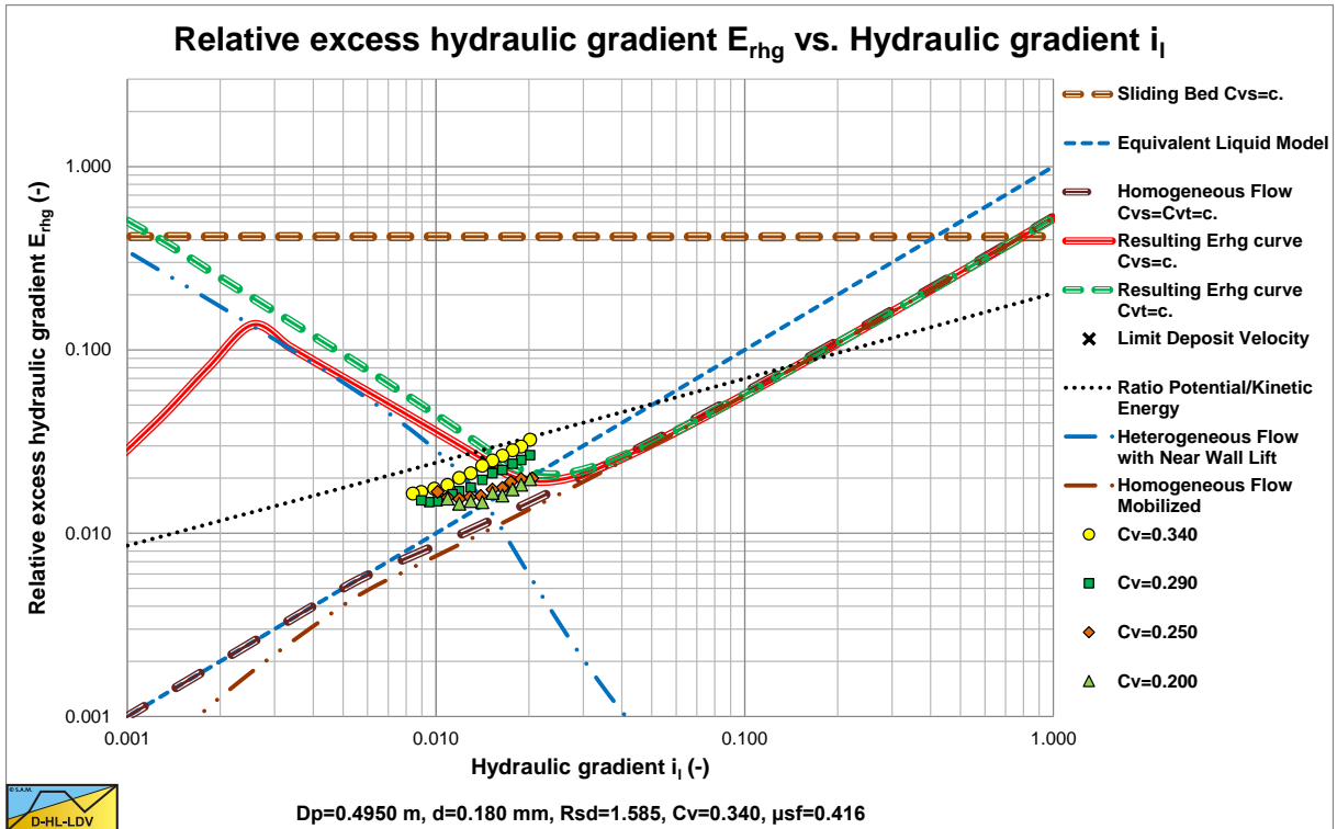
Figure 6.22-15: Data of Gillies (1993) in a large diameter pipe D_p=0.495 m and small particles d=0.18 mm.
