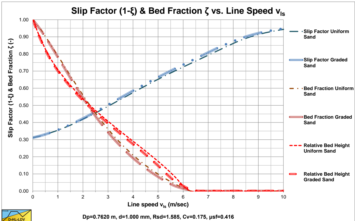
Figure 7.13-20: Slip factor, bed fraction and bed height for d_{50}=1.0 mm and D_p=0.762 m.
