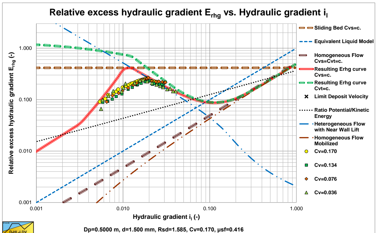
Figure 6.14-7: The relative excess hydraulic gradient of the Kazanskij (1980) experiments.
