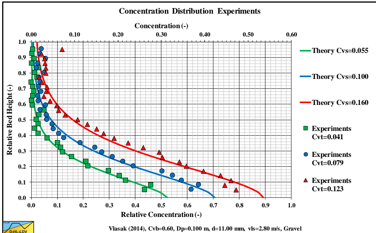
Figure 15.7-40: Vlasak et al. (2014) d=11.0 mm, D_p=0.1000 m, v_{ls}=2.8 m/s.
