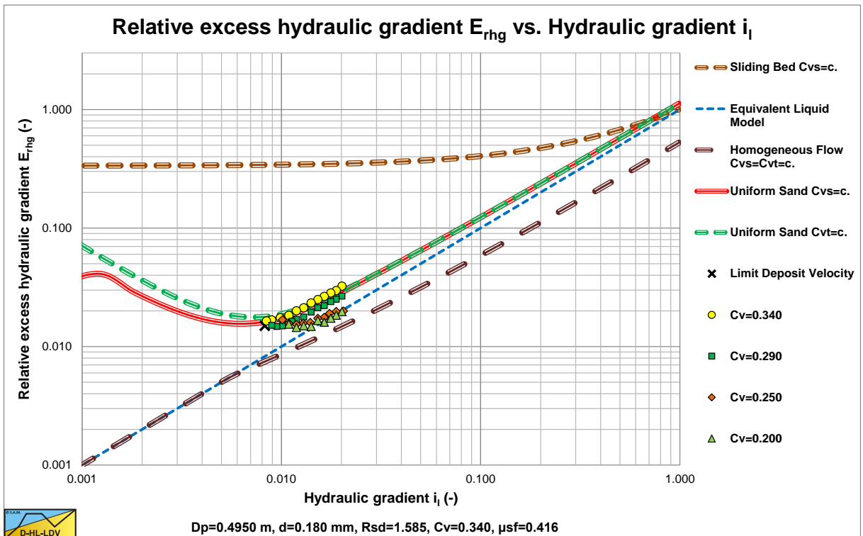
Figure 6.22-16: Data of Gillies (1993) in a large diameter pipe D_p=0.495 m and small particles d=0.18 mm, including Thomas (1965) viscosity.
