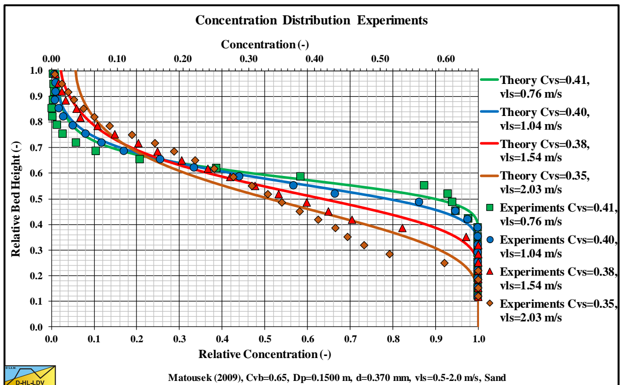
Figure 15.7-38: Matousek et al. (2009) d=0.370 mm, D_p=0.1500 m, v_{ls}=0.5-2.0 m/s.
