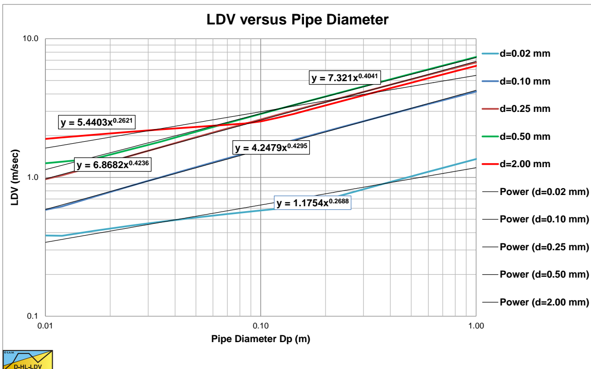
Figure 15.5-8: The Limit Deposit Velocity versus the pipe diameter for 5 sands.
