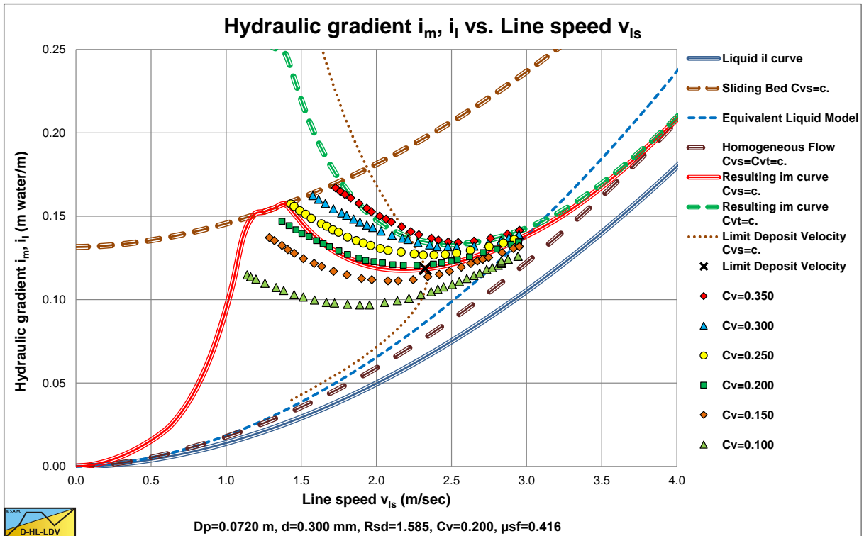
Figure 6.2-5: Sand with d=0.30 mm in a 0.072 m diameter pipe. Data points of Siegfried (Durepaire, 1939) reconstructed from fit lines (source (Westendorp, 1948)).
