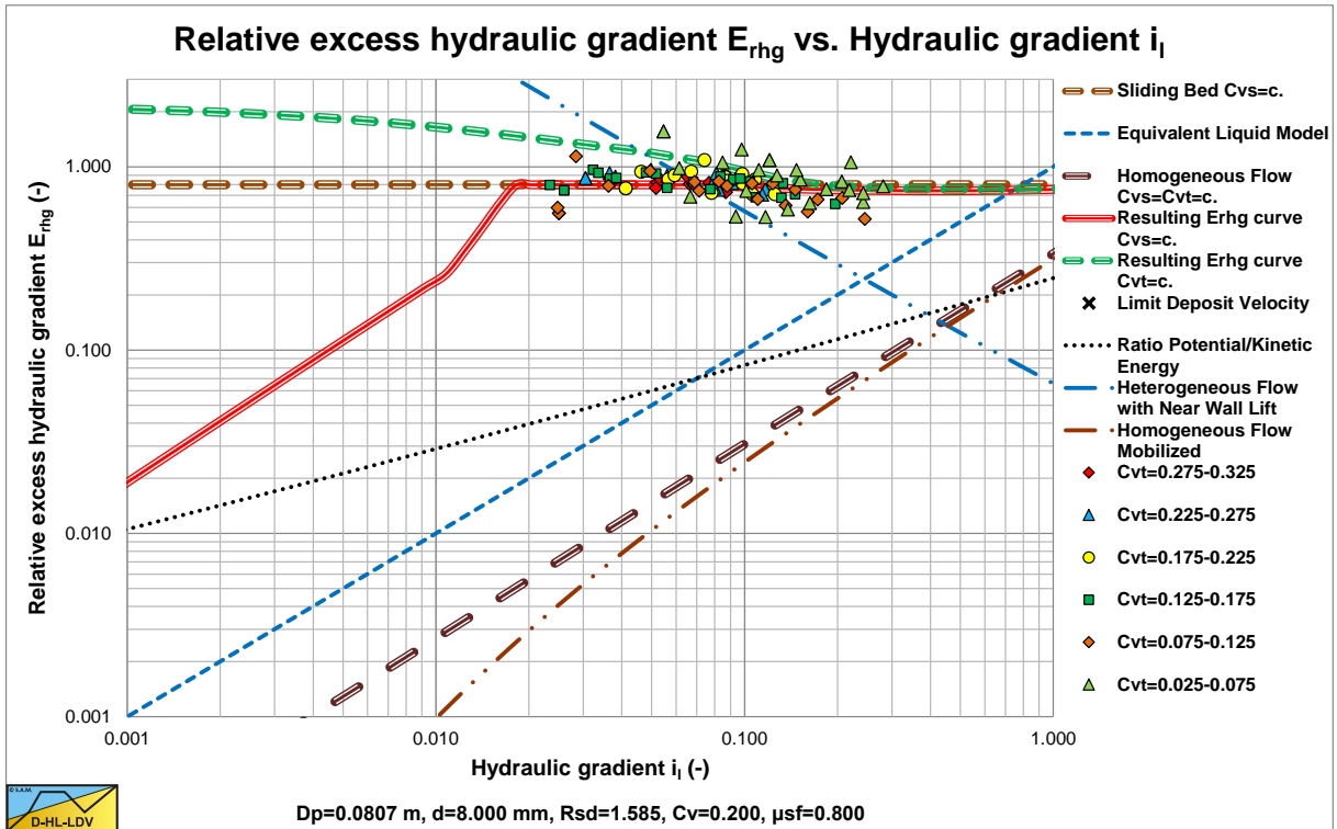
Figure 6.11-5: The Yagi et al. (1972) experiments with gravel and spatial concentration.
