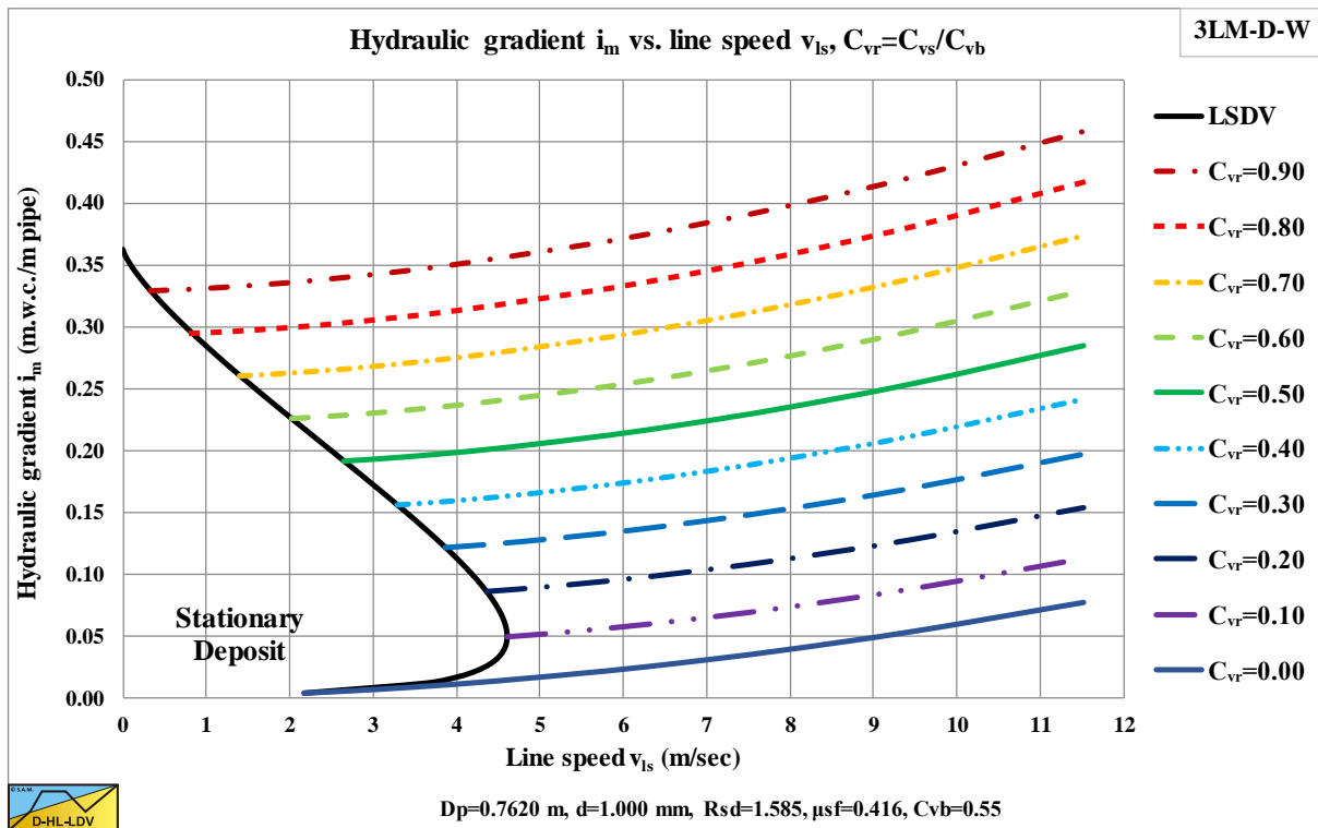
Figure 7.4-29: The hydraulic gradient i_m versus the line speed v_{is} , C_{vr}=C_{vs}/C_{vb} . The submerged weight approach, with sheet flow.
