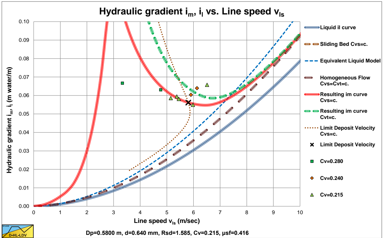
Figure 6.4-3: Experiments with sand d=0.64 mm and a pipe diameter of D_p=0.58 m.
