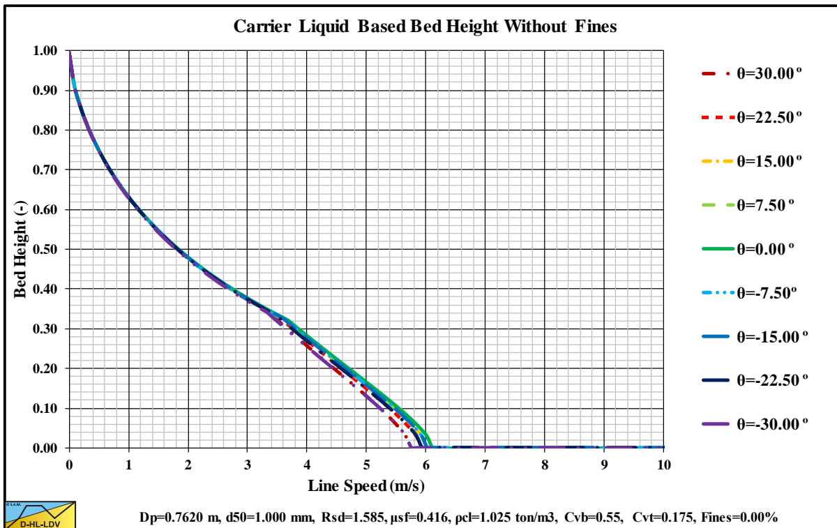
Figure 15.5-42: The bed height for 9 inclination angles.
