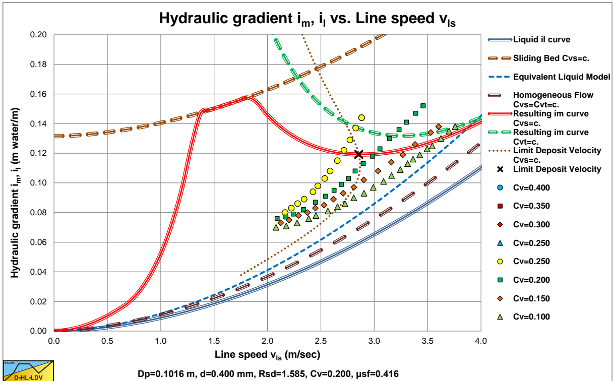
Figure 6.2-4: Sand with d=0.4 mm in a 4 inch diameter pipe. Data points of Howard (1938) reconstructed from fit lines (source (Westendorp, 1948)).
