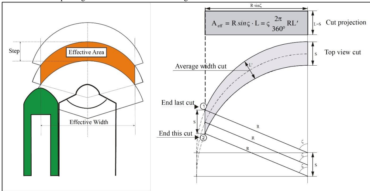
Figure 12-5: The effective dredging area.
