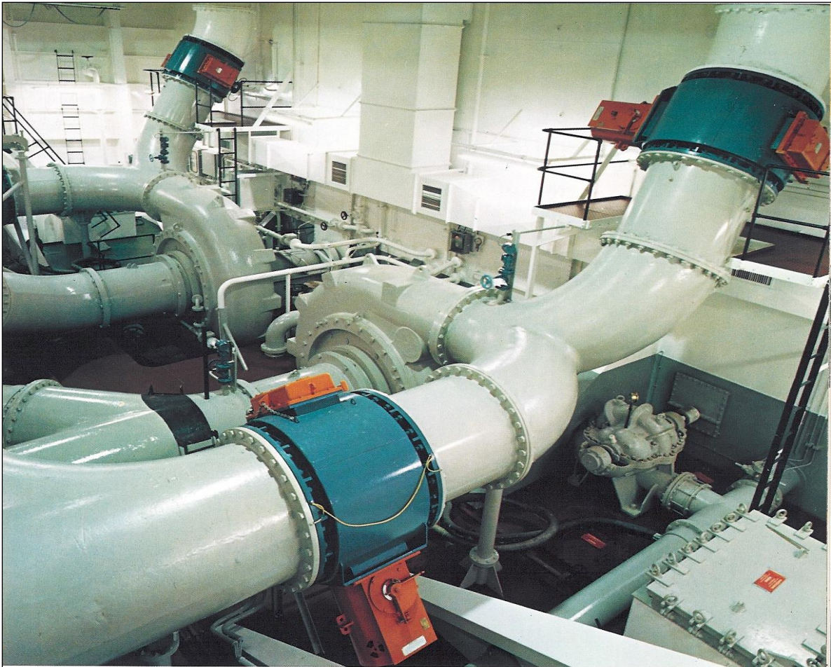
Figure 8-3: Centrifugal pumps.
